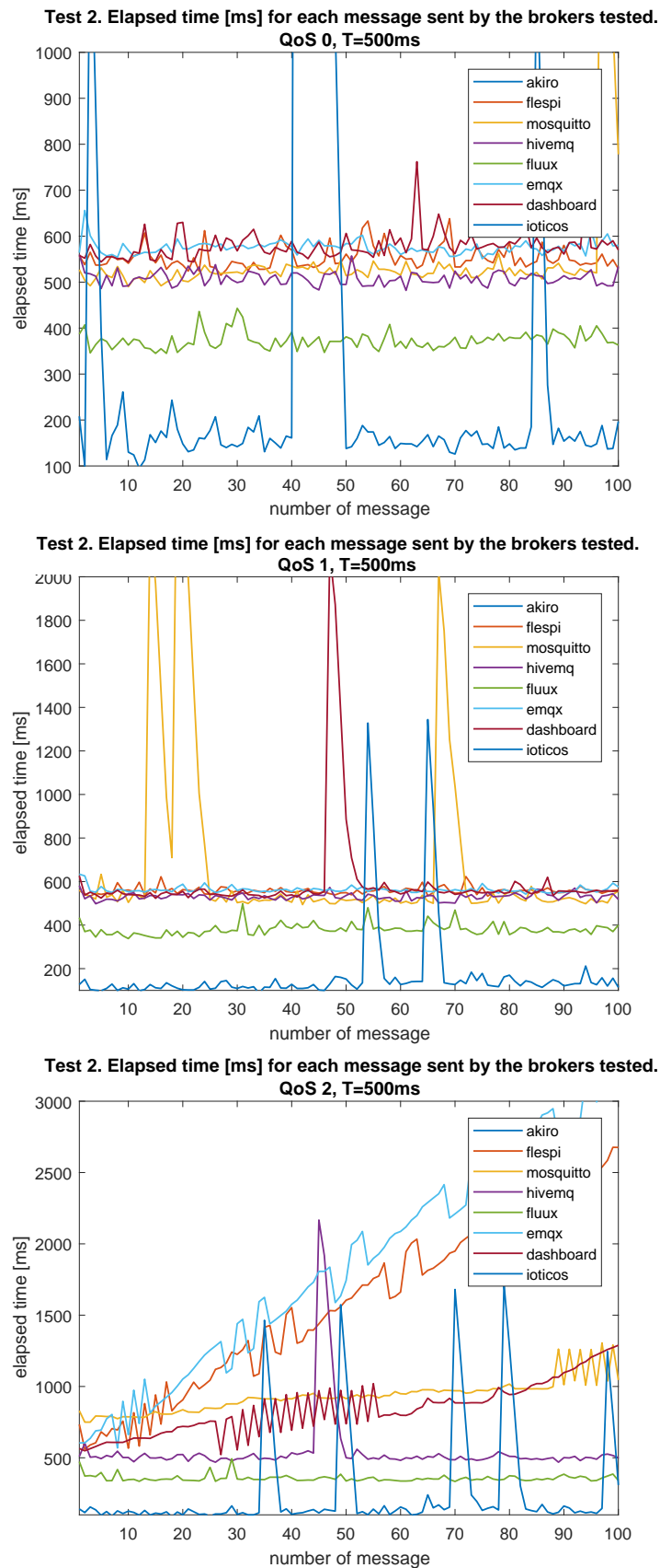
Fig. 4: Elapsed times of 100 messages sent by the brokers tested in ASSE, ISSN 2454-7496, Page 13
